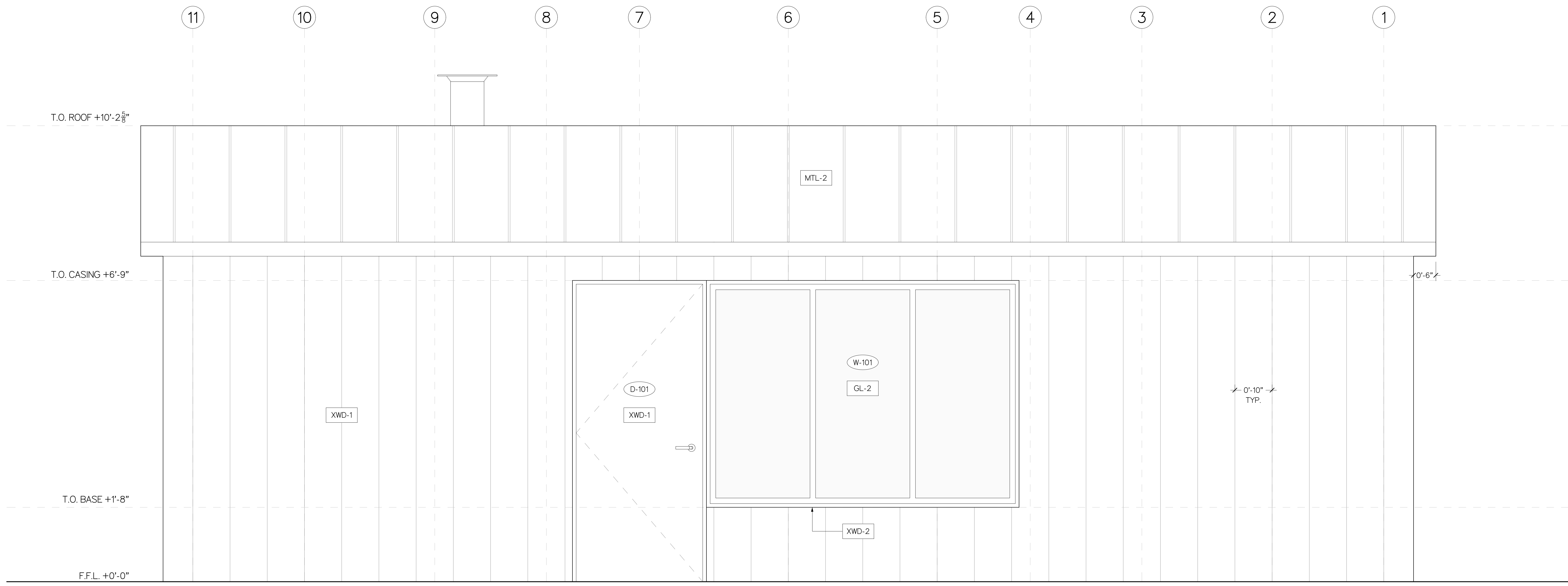
1 NORTH ELEVATION
